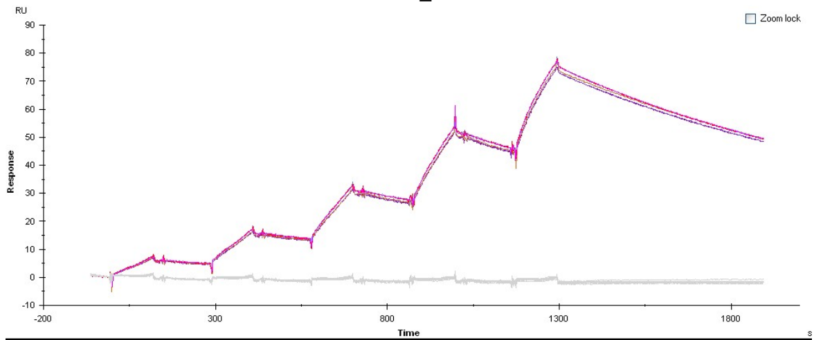
Fig A.1: Overlay of six consecutively recorded single cycle kinetics (SCK1)
