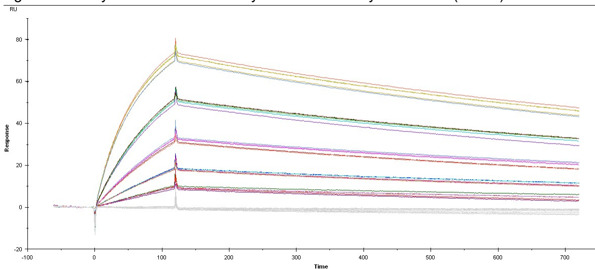
Fig A.1: Overlay from six consecutively recorded multi cycle kinetics (MCK1)
