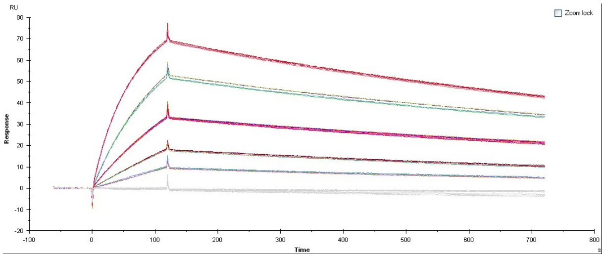
Fig A.1: Overlay from six consecutively recorded multi cycle kinetics (MCK1)
