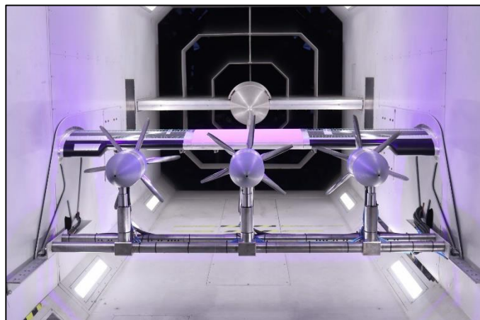
Figure 1: Distributed propulsion test case in the wind tunnel.
