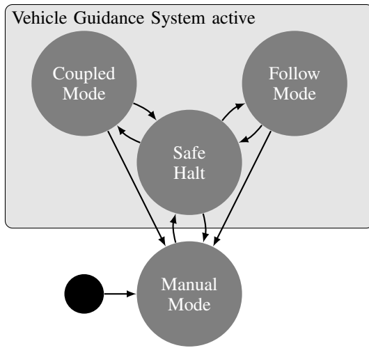
Fig. 2. Modes of Operation of the Planned System
