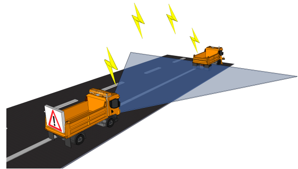
Fig. 1. Principle System Set-up of a Unmanned Protective Vehicle with a Road Maintenance Vehicle in Front
