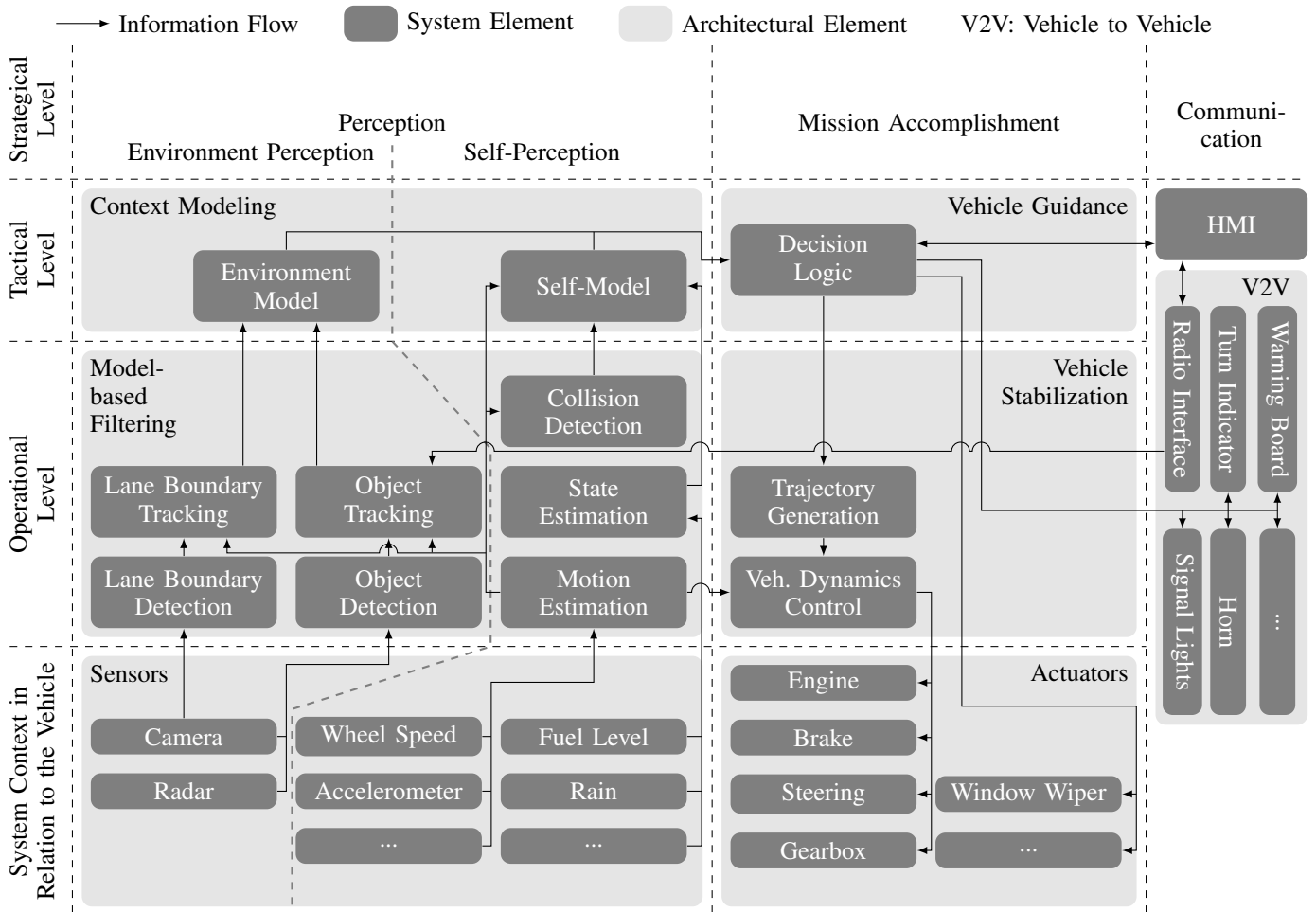
Fig. 3. Functional System Architecture of the Planned System with Information Flow
