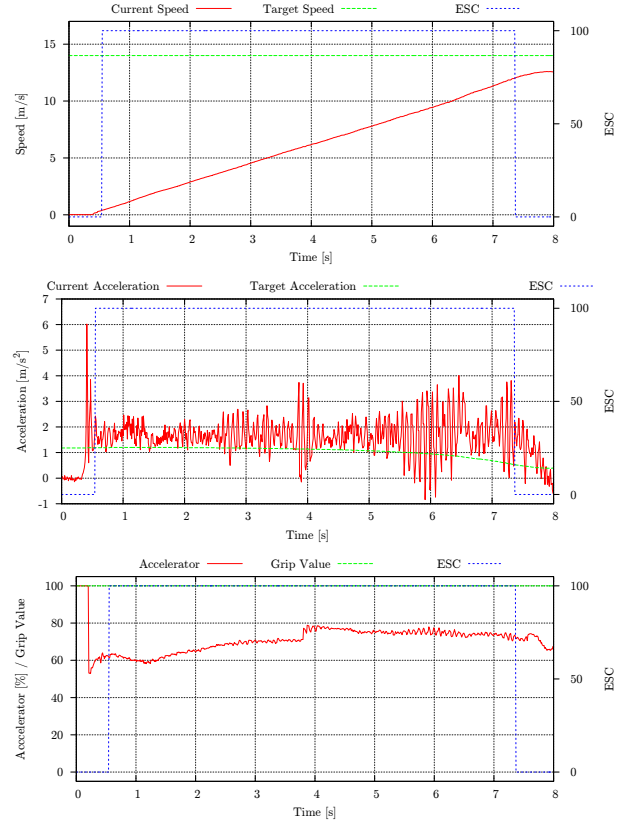
Fig. 4. Speed, Acceleration and Grip Level without Grip Value
