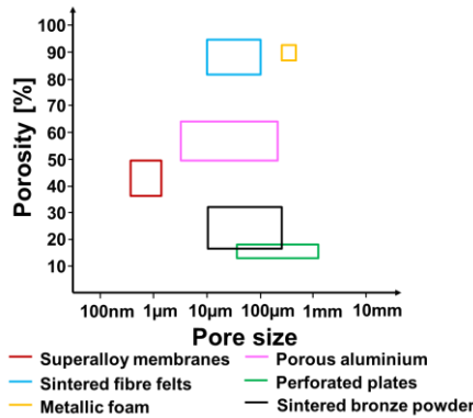
FIGURE 10. Overview of investigated surface materials
