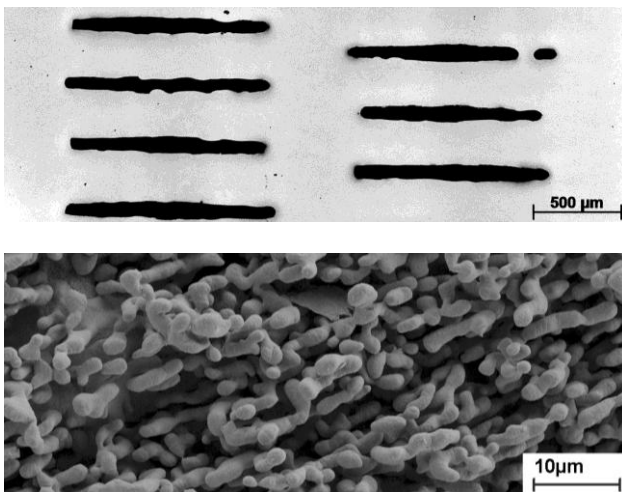
FIGURE 11. Surface Materials with nonisotropic permeability
