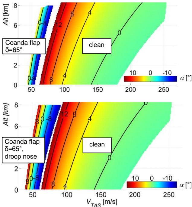
FIGURE 19. Trimmed flight envelopes for Reference Configuration with and without high-lift setting: Fixed nose (upper part) and morphing droopnose (lower part)
