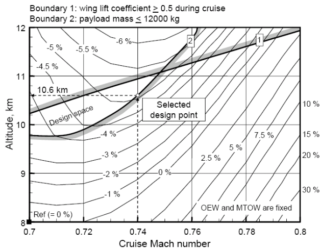
FIGURE 3. Effect of Mach number and Altitude on DOC
