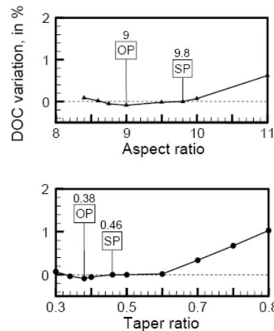
FIGURE 5. Optimization of wing planform parameters (SP - starting point, OP - selection for SFB 880 Reference Configuration)
