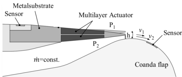
FIGURE 16. Concept sketch of integrated flow actuator and sensors for pulsed blowing and closed-loop control
