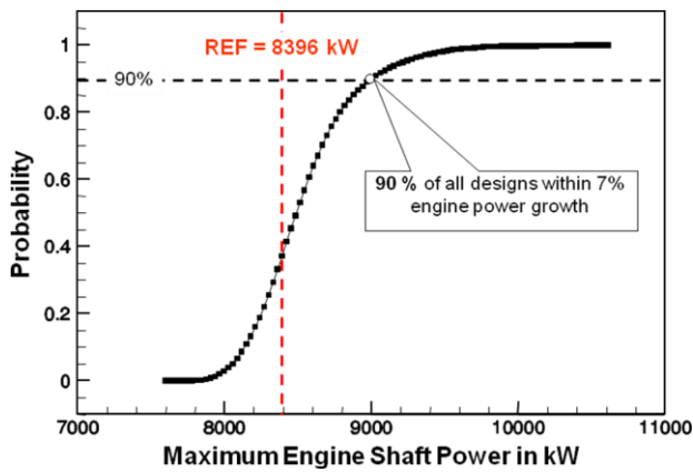
FIGURE 7. Engine growth over all design samples
