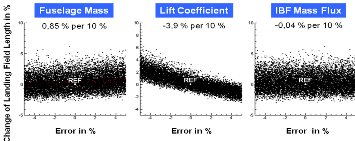
FIGURE 6. Effects of fuselage mass, lift and blowing mass flux errors on landing field length
