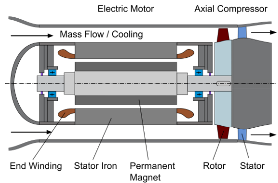
FIGURE 15. Motor integration in compressor concept
