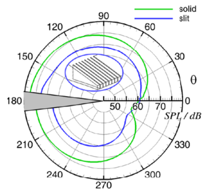
FIGURE 9. Computed measure of trailing edge noise emissions for solid and slit edges
