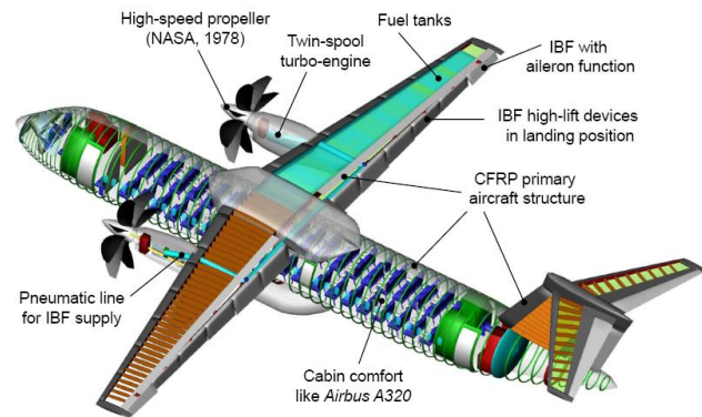
FIGURE 1. SFB 880 Reference Configuration
