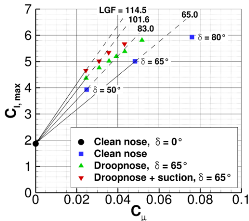
FIGURE 13. Lift gains versus blowing momentum obtained by droopnose and combined suction and blowing approaches ( \delta – deflection angle of flap)
