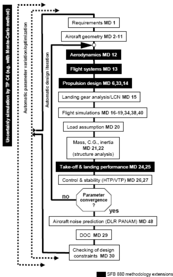
FIGURE 2. Schematic of Preliminary Aircraft Design with PrADO with design modules (MD)
