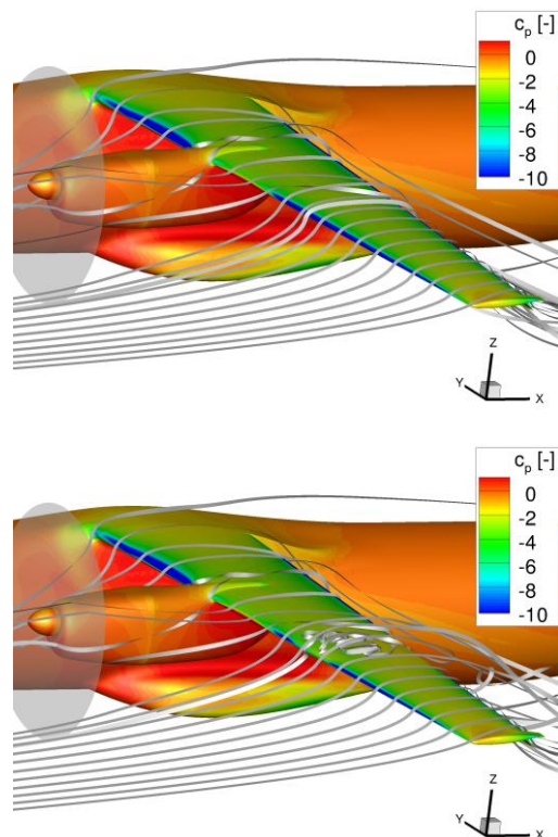
FIGURE 18. RANS simulation of wing stall of complete Reference Configuration with Coanda flaps at \delta=65^\circ and c_{\mu}=0.033 on wing: \alpha=2^\circ below stall (upper part) and \alpha=3^\circ beyond stall (lower part)
