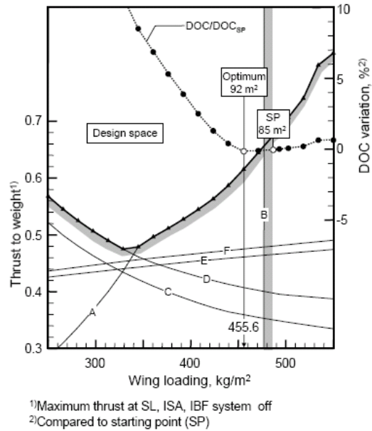
FIGURE 4. Variation of thrust-to-weight ratio and DOC over wing loading.
