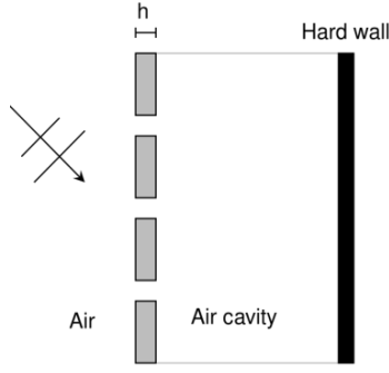
Fig 22. Perforated plate mounting configuration.
