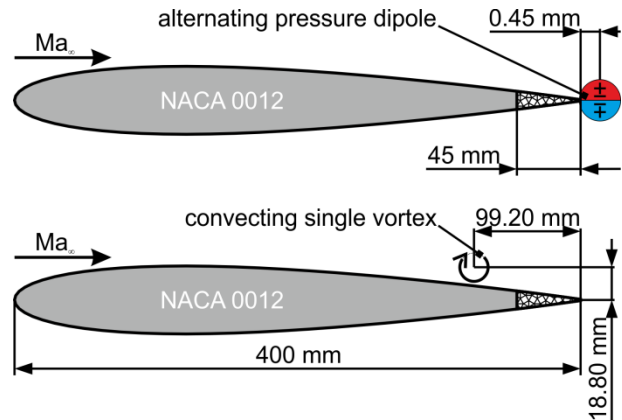
Fig 3. Numerical implementation of the edge dipole (top) and the advecting single vortex (bottom), see also [3].
