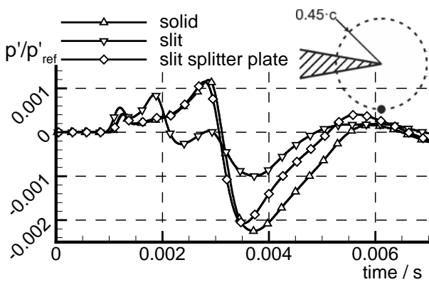
Fig 6. Time signal of the fluctuating pressure at a micro-phone position 90^\circ below the trailing edge during the passage of a single vortex, p'_{ref} = \rho_\infty U_\infty v'_{max} where v'_{max} — max. speed perturbation induced by initial vortex.
