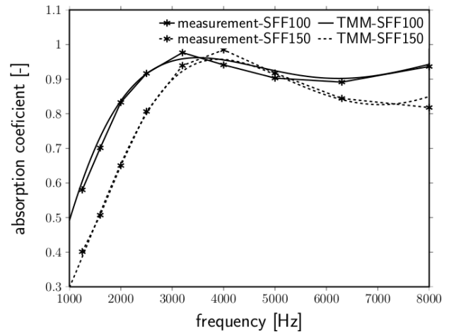
Fig 21. Absorption coefficient. Sintered fibre felts.
