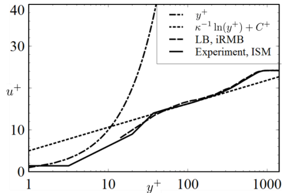
Fig 11. Time-averaged streamwise velocity profile at 95% of plate's chord in inner coordinates (designated with +).
