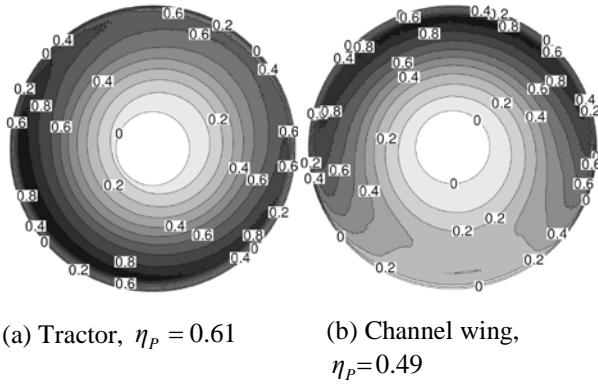
Fig 17. Propeller disk distributions of relative thrust t/t_{max} at constant shaft power coefficient.
