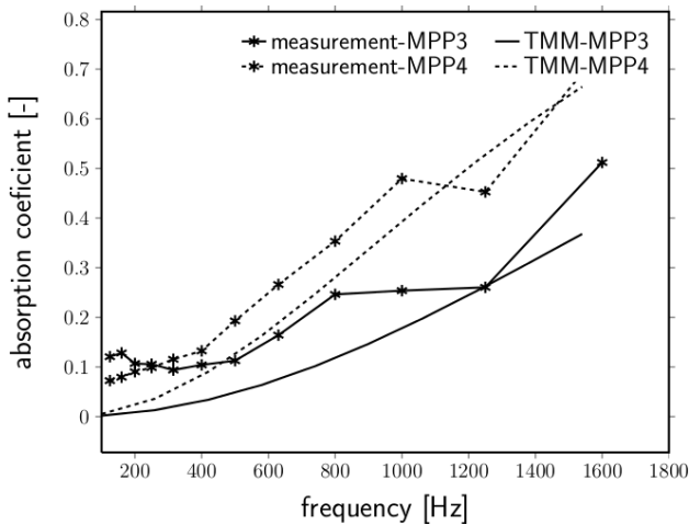
Fig 23. Absorption coefficient. Perforated plate.
