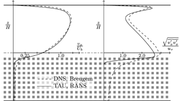
Fig 8. Comparison of results of partially porous channel flow. DNS against the newly implemented TAU-implementation.
