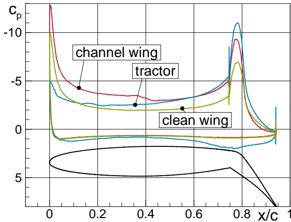
Fig 18. Pressure distribution at midspan.
