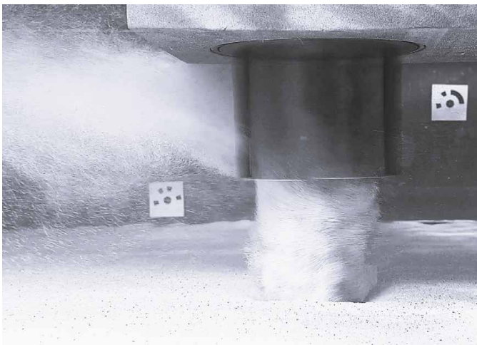
Voith-Schneider Propeller induced vortex with suspended sand and transport of the suspended material in the wake flow field Source: C. Schwartpaul (LWI)
